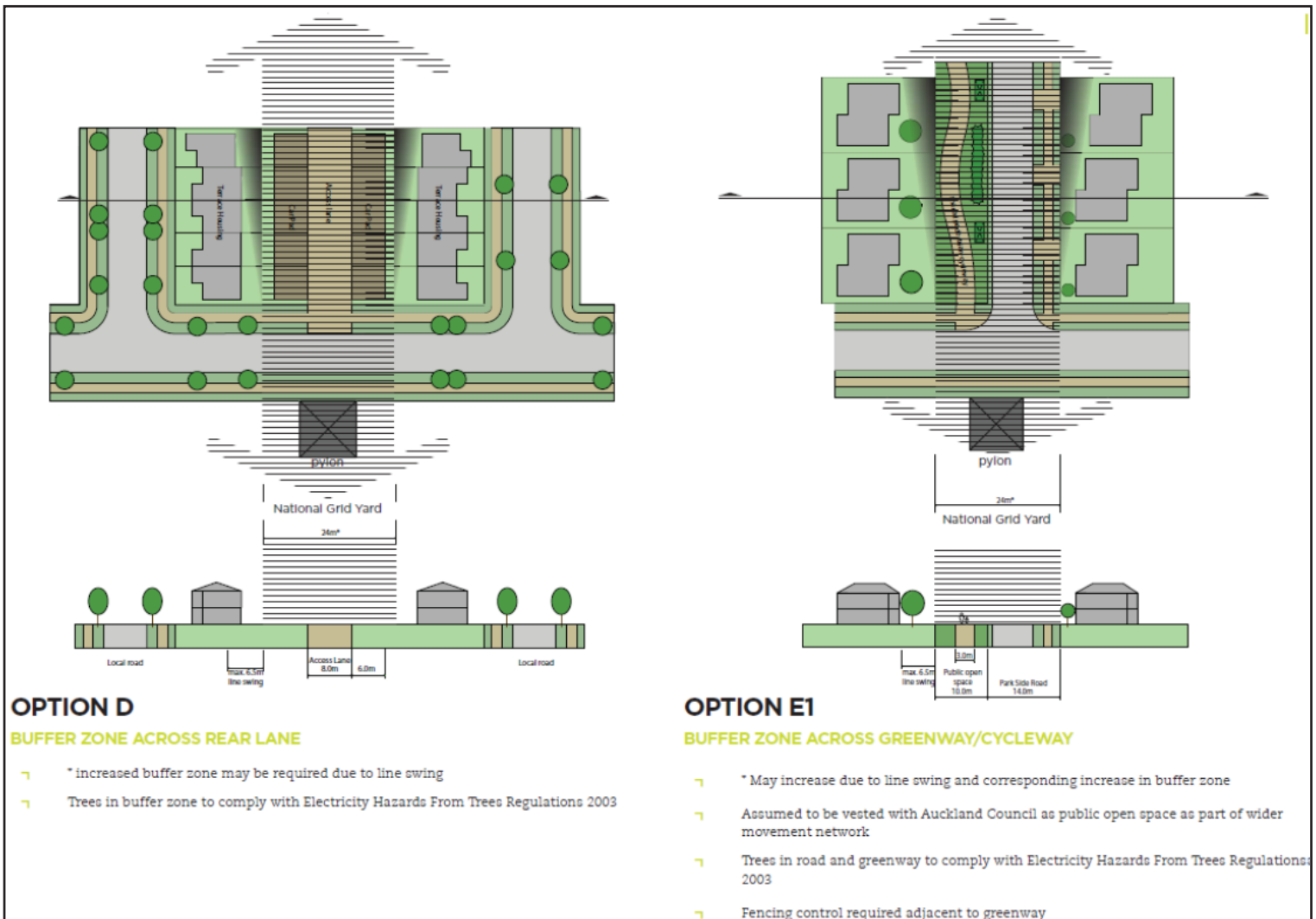
Figure 13. Possible design options for subdivision layouts within the National Grid Subdivision Corridor - Option D and E1
